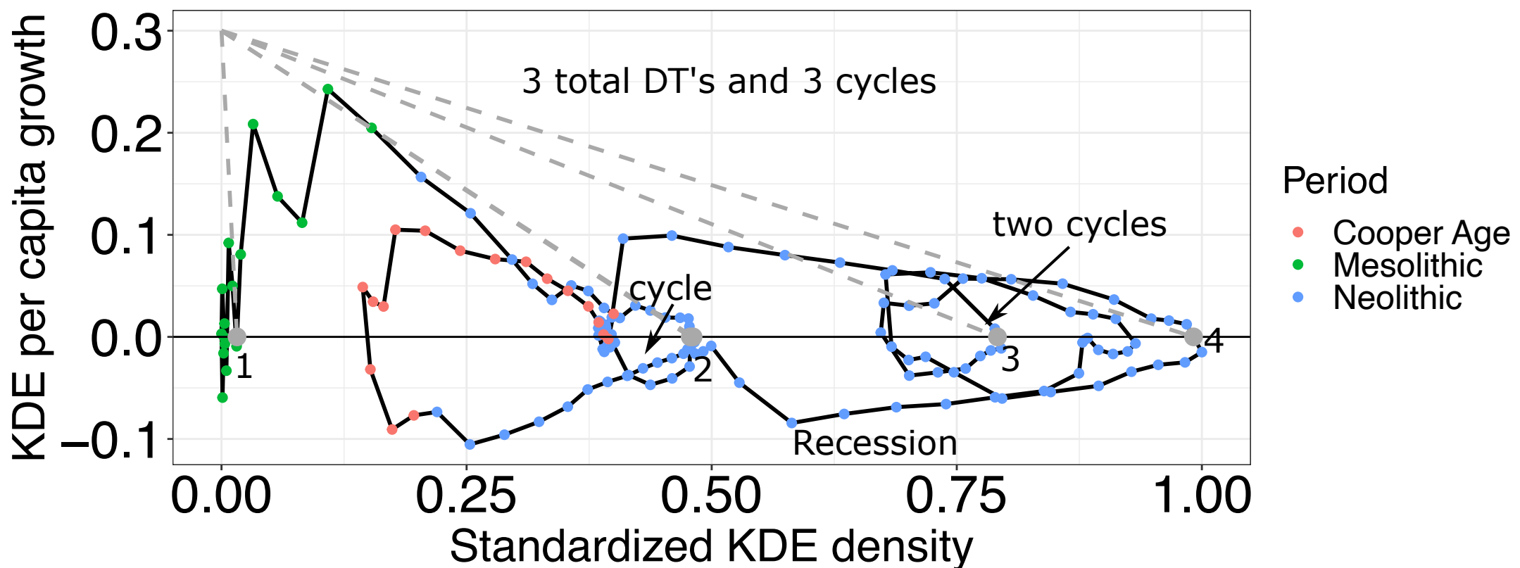
(C) KDE Per Capita Growth vs. Density – Greece (23)
